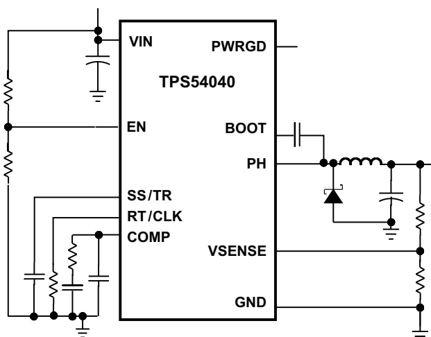
SIMPLIFIED SCHEMATIC
