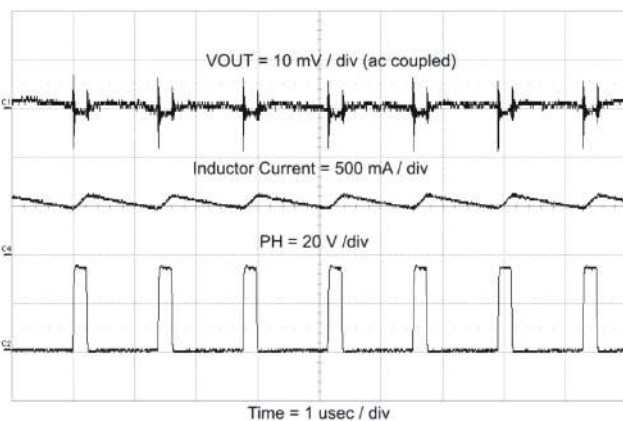
Figure 53. Output Ripple CCM
