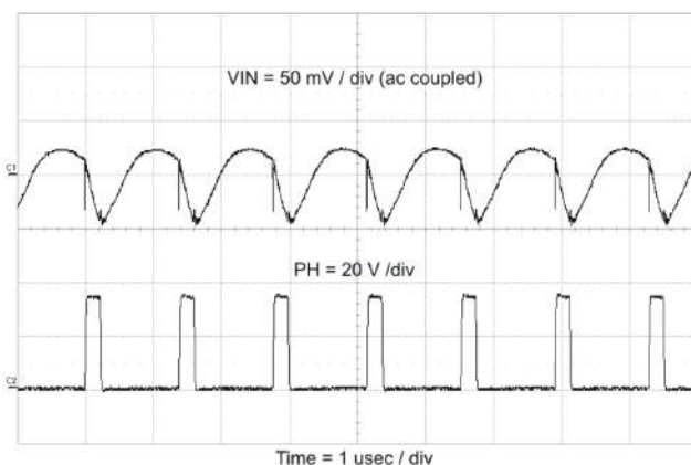
Figure 56. Input Ripple CCM
