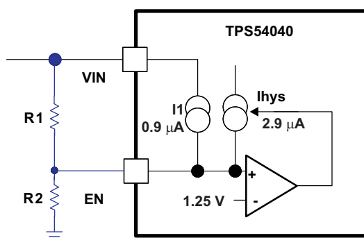
Figure 28. Adjustable Undervoltage Lockout (UVLO)
