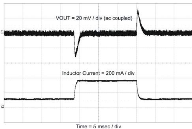
Figure 51. Load Transient
