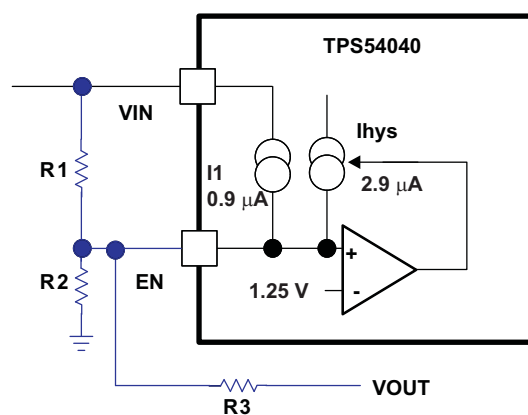
Figure 29. Adding Additional Hysteresis
