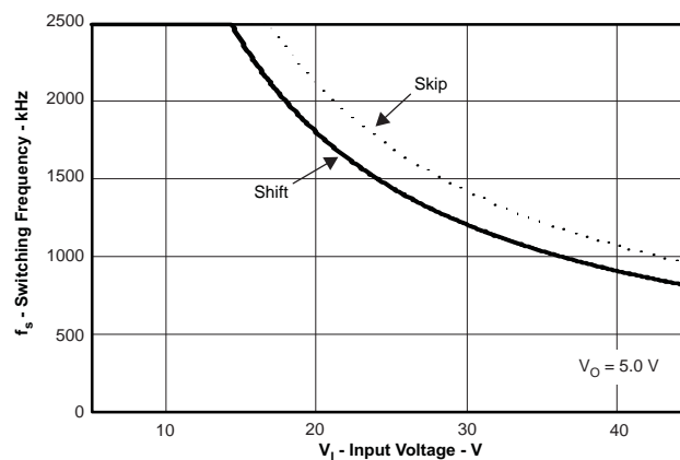
Figure 41. Maximum Switching Frequency vs. Input Voltage
