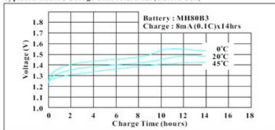
Typical Quick Charge Characteristics (Button Cell)
