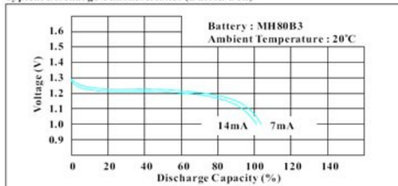
Typical Discharge Characteristics (Button Cell)
