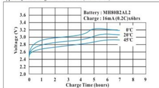
Typical Quick Charge Characteristics (Button Cell)
