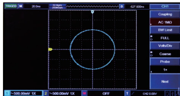
Lissajous figure phase measurement
