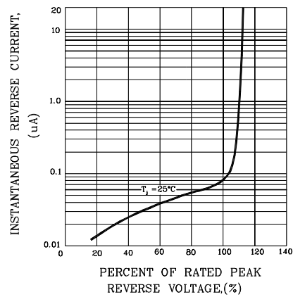
FIG.4-TYPICAL REVERSE CHARACTERISTICS
