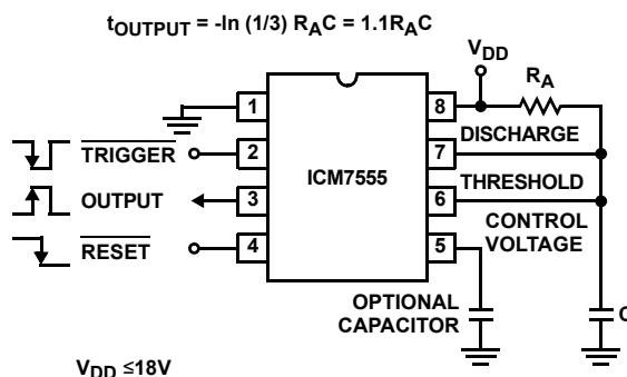
FIGURE 6. MONOSTABLE OPERATION
