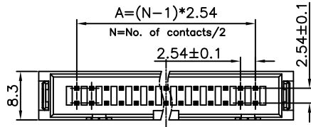
W/O SCREW HOLE
