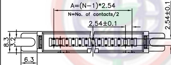
W/ SCREW HOLE
