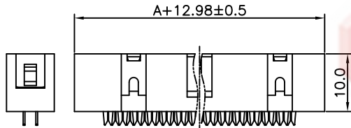
W/O SCREW HOLE
