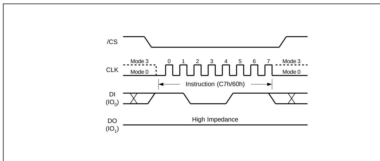
Figure 34. Chip Erase Instruction
