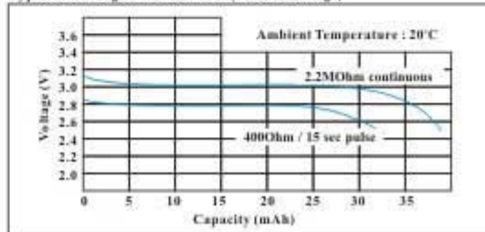
Typical Discharge Characteristics (Pulse Discharge)
