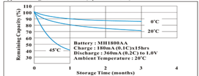
Typical Storage Characteristics (Cylindrical Cell)
