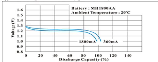
Typical Discharge Characteristics (Cylindrical Cell)
