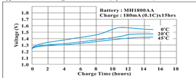
Typical Quick Charge Characteristics (Cylindrical Cell)
